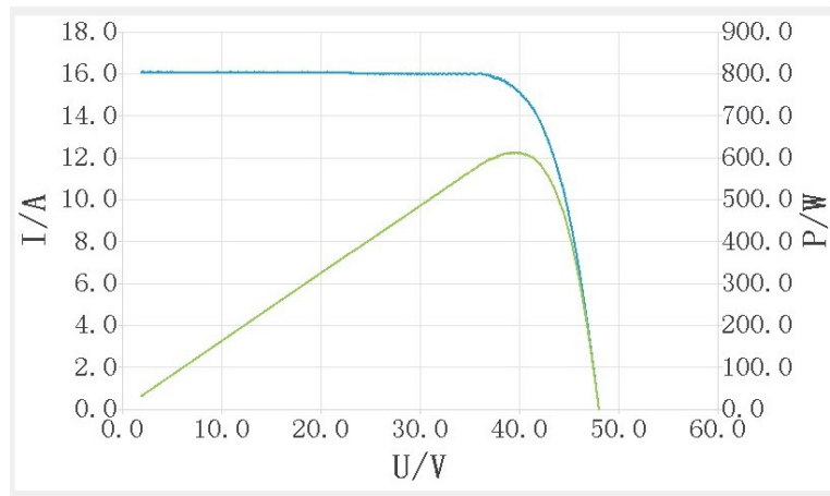
Fig. 5 IV curve of module No.1 Serial number: AS29200100001
